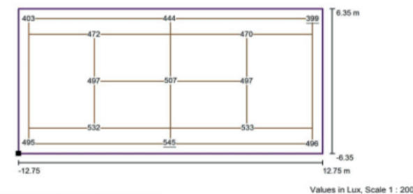
Campo Haillet 6 lamps / Tennis 1 Calculation Grid (PA) / Value Chart (E, Horizontal)
